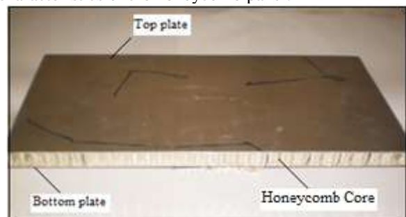
Fig.1 Honeycomb sandwich structure
