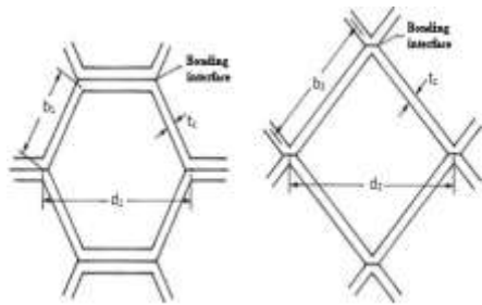
Fig.4 (a) Right hexagonal cell. (b) Square cell Two-dimension model of Honeycomb Sandwich Structure
