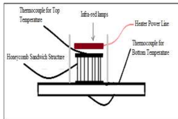
Fig. 19 A Schematic of the Experimental Model
