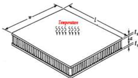
Fig.6 Honeycomb sandwich thermal protection system (TPS) subjected to heating over entire upper surface.
