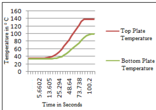
Fig.25 Experimental values for aluminum honeycomb sandwich structure
