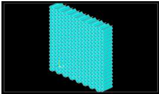
Fig.9 Pattern of Hexagonal Honeycomb Cells
