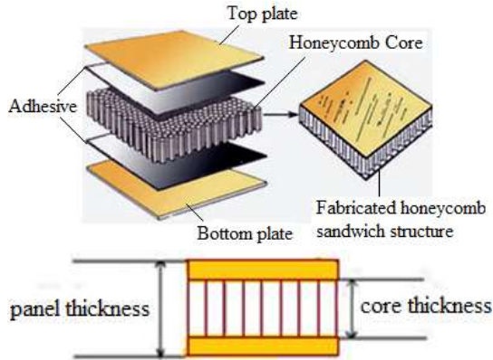
Fig. 2 Exploded view of honeycomb core sandwich structure
