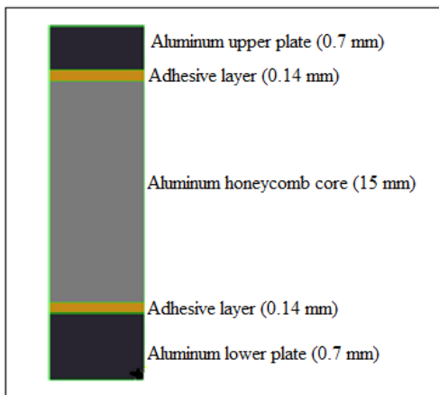
Fig.5 Two-dimension model of Honeycomb Sandwich Structure
